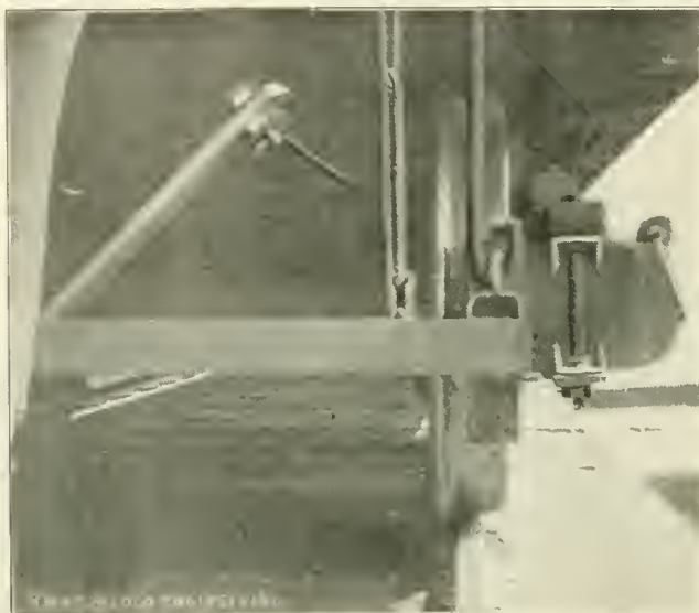
THE REASON WHY SOME BRAKE SHOES WEAR UNEVENLY AND PRODUCE FLANGES.
